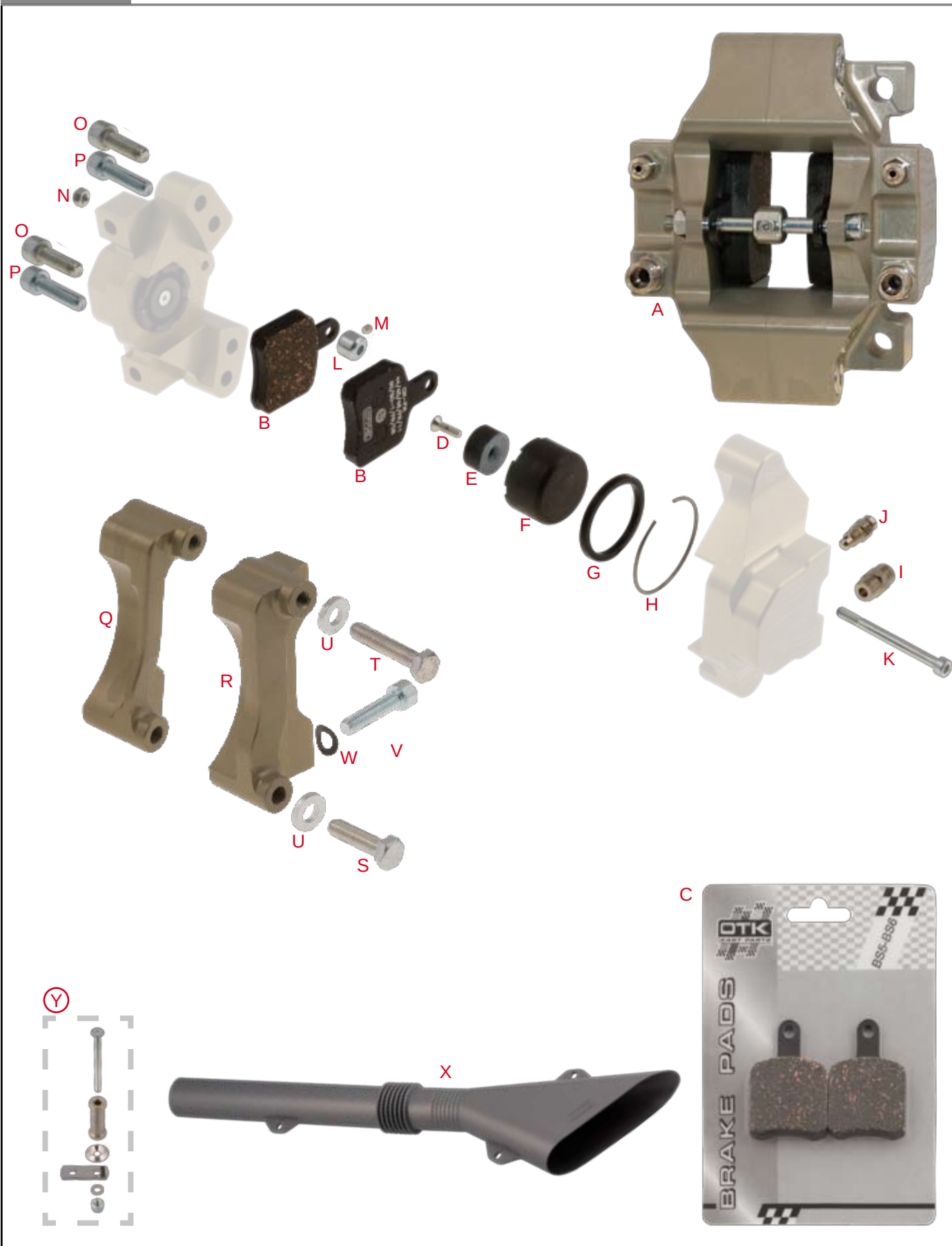
Tav. 33 PINZA FRENO POSTERIORE • REAR BRAKE CALIPER BS6
